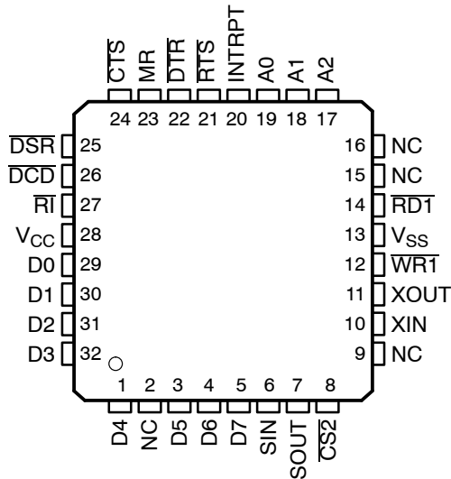
RHB PACKAGE (TOP VIEW)
